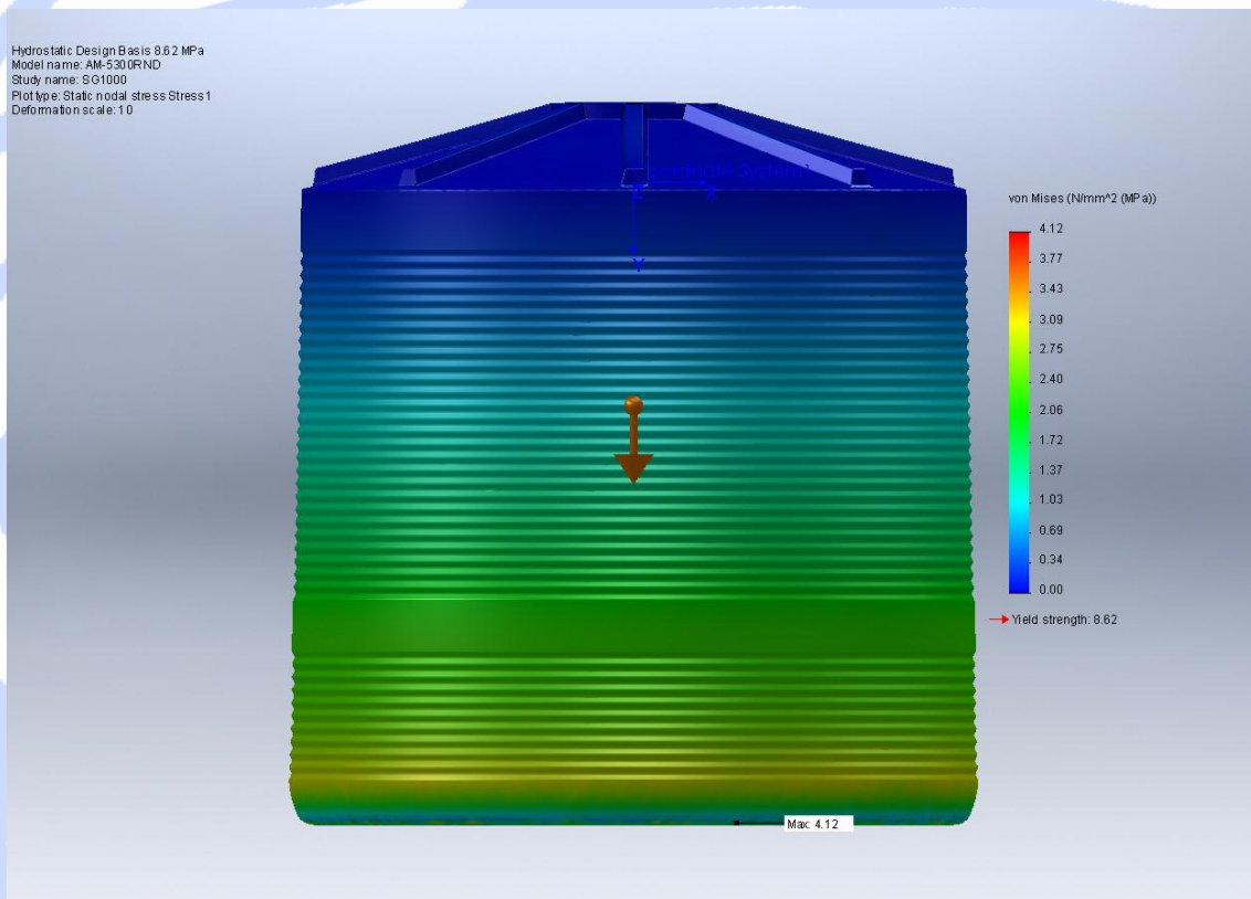
Stress analysis diagram
